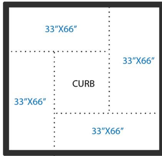
Large Standard Unit - 99"x99"
